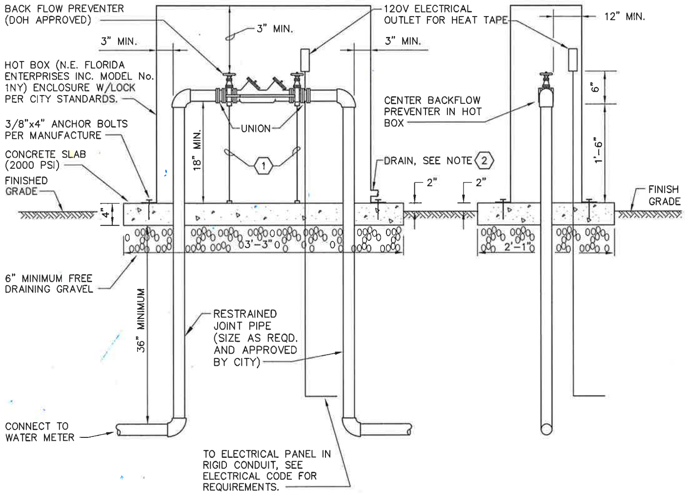
REDUCED PRESSURE BACKFLOW DEVICE NOT TO SCALE
