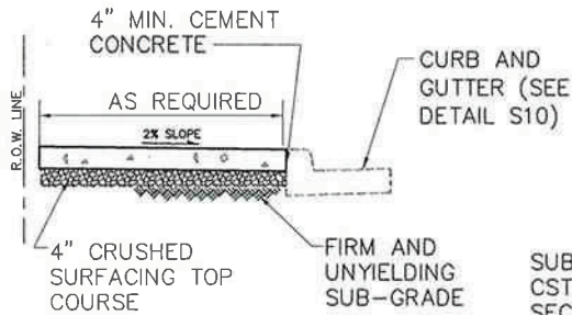
TYPICAL SECTION
