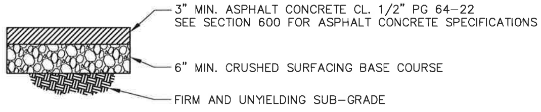
MIN. PAVEMENT SECTION SECTION A NO SCALE
