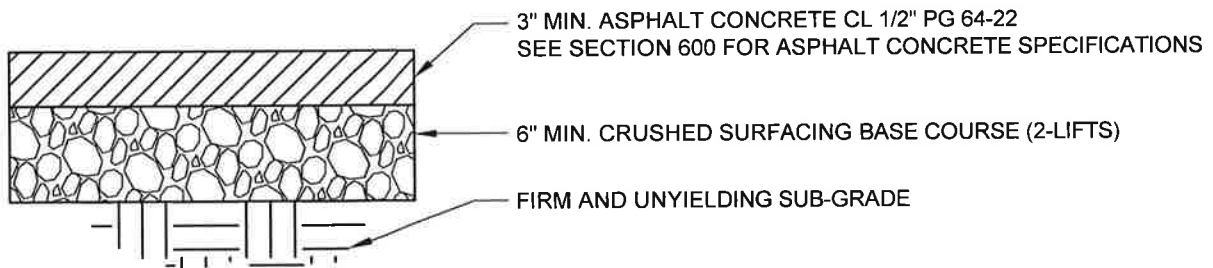
MIN. PAVEMENT SECTION SECTION A NO SCALE
