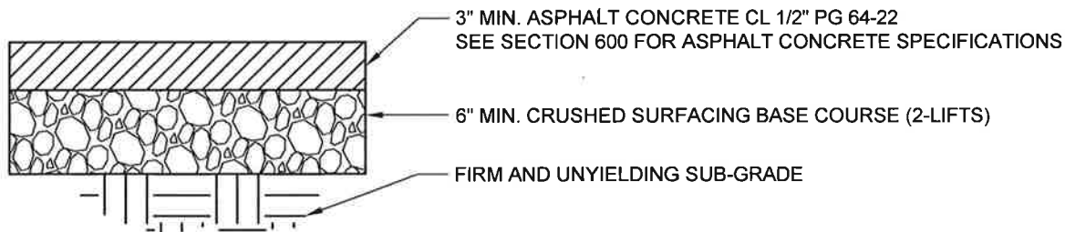
MIN. PAVEMENT SECTION SECTION A NO SCALE
