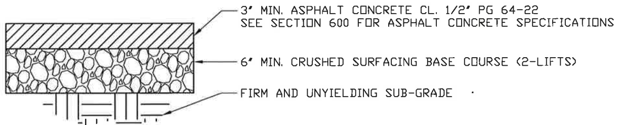
MIN. PAVEMENT SECTION SECTION A NO SCALE
