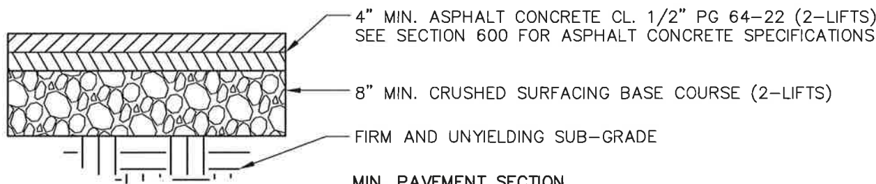
MIN. PAVEMENT SECTION SECTION A NO SCALE
