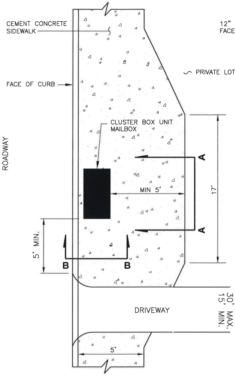
PLAN VIEW
